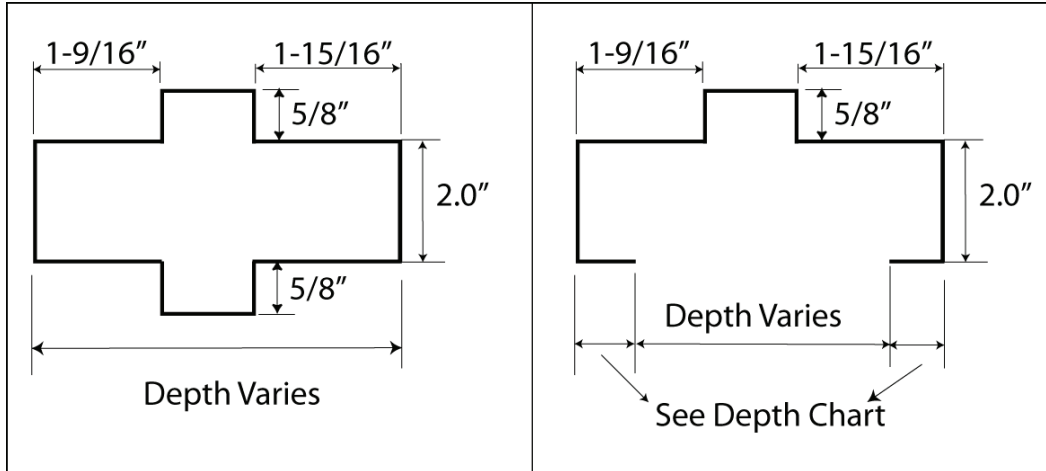
Mullion
