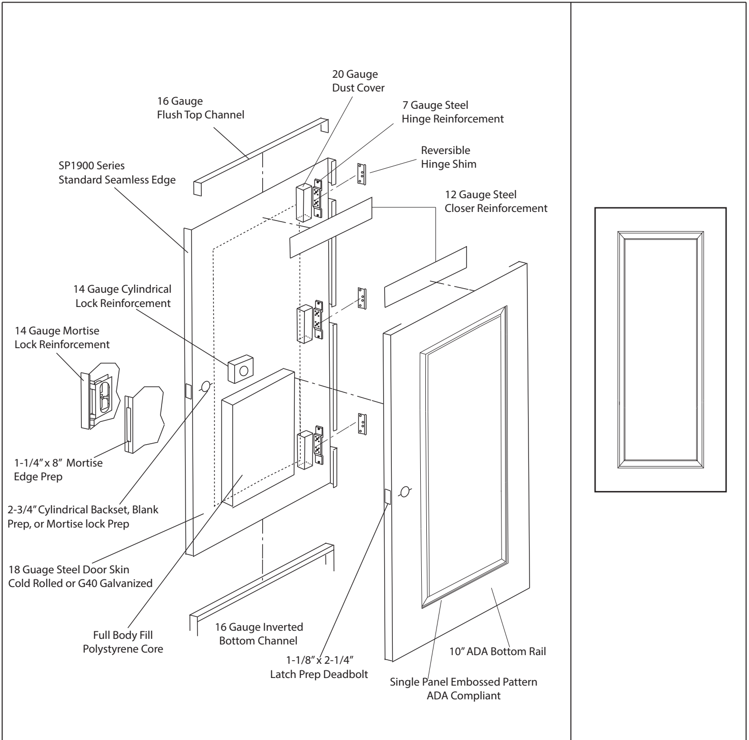
SP1900 Series, Single Panel Door, Sound Rated, 18-Gauge, STC 28
